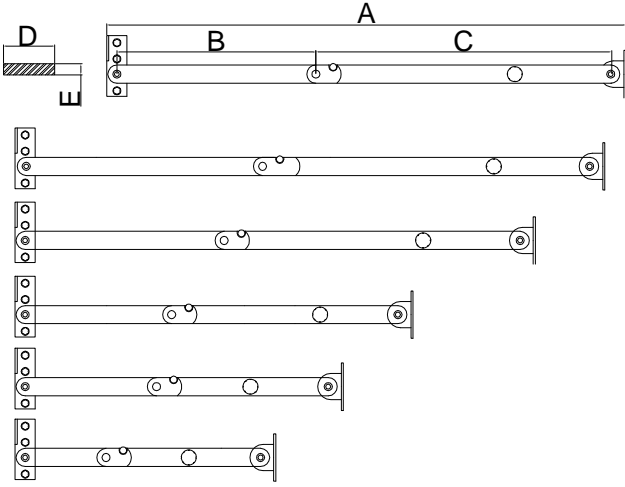
PANJUR MAKASI SHUTTER BEND SCISSORS GROUP
