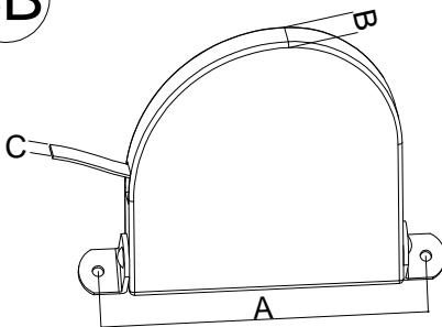
BORA 2 OTOMAT K MAKARA BORA 2 SHUTTER PULLEY
